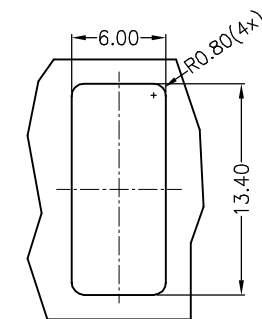
MOUNTING PANEL CUTOUT (INTERNAL SIDE)
